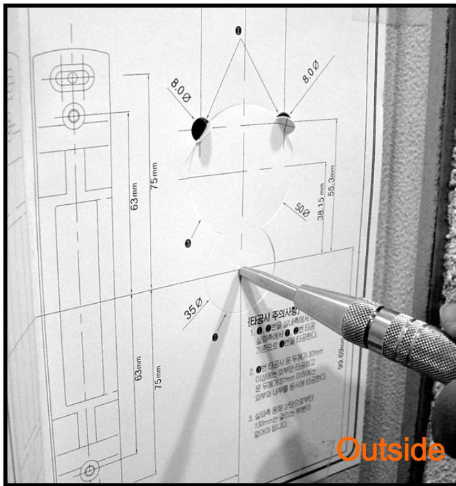
5. At outside, After locating the 8mm hole with Installation guide paper's 8mm hole location, Punching & Marking 35mm's Hole & 50mm's Hole
