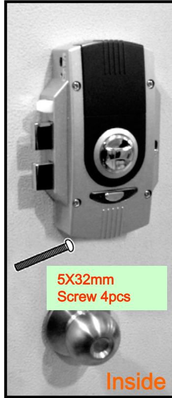
12. Fix up Inner lock body at inner plate with the screws (4pcs)
