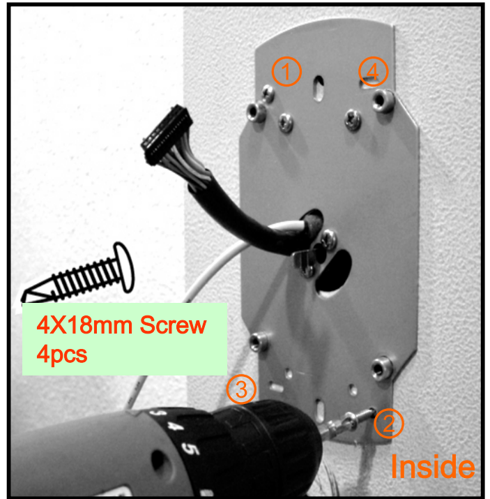
10. Fix up Inner plate and inside door with the screws (4pcs)
