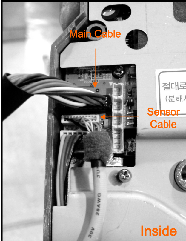
11. Connect Sensor cable & Main Cable
