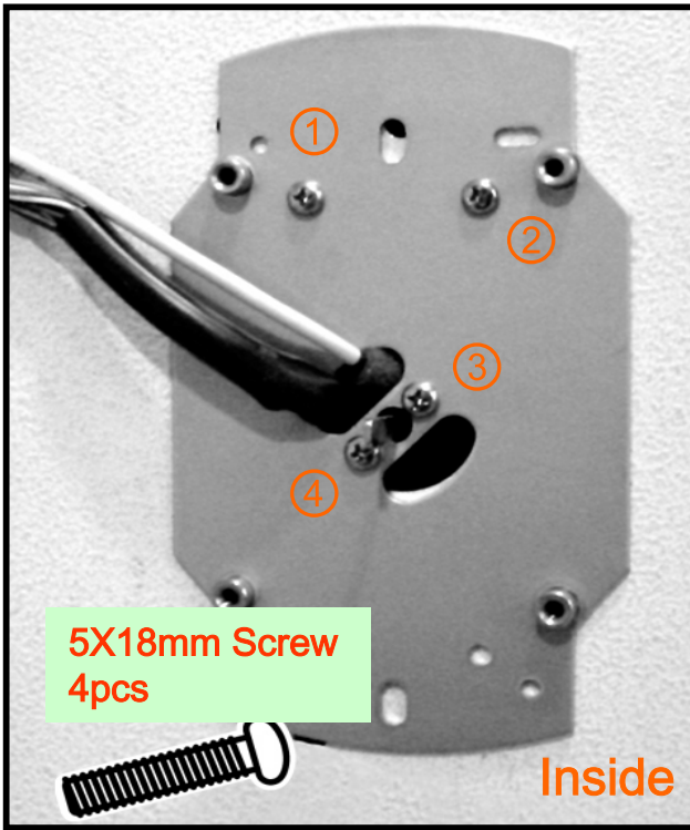
9. From Inside, Place a plate at the inside door, then, combine the plate and the front body with the screws (4pcs)
