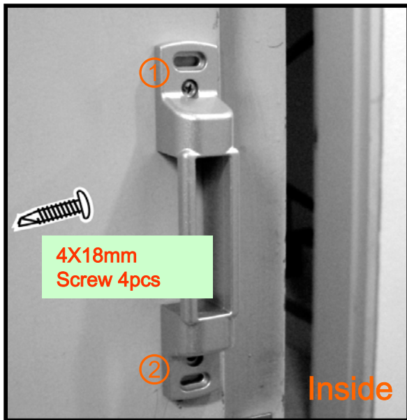
13. Fix up the lock bracket
