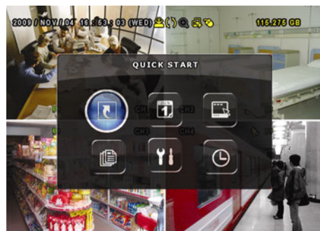
Main Menu
